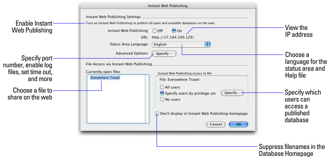
FileMaker Pro Instant Web Publishing dialog box
